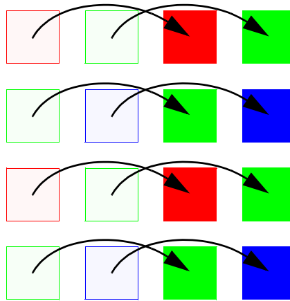
Figure 45: 2 × horizontal binning (Guppy PRO F-503B, F-503C)
